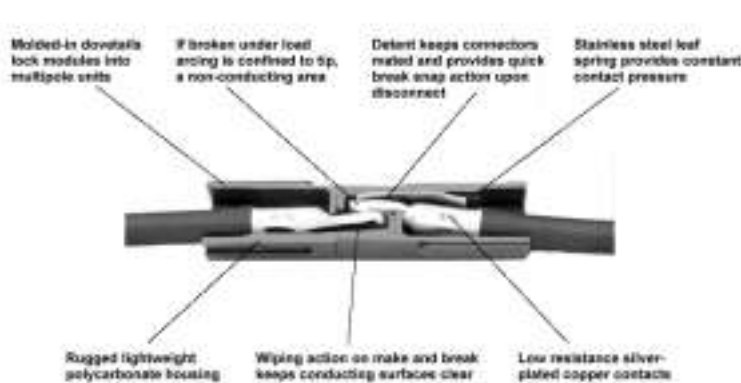
Photograph 37: This is how the two housings and the two contacts snap together to give a secure very low resistance connection.
