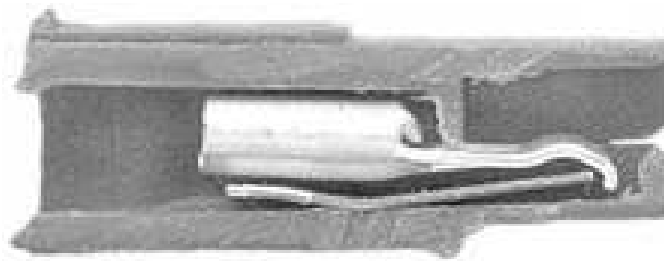
Photograph 36: This is how the contact locks over the spring.
